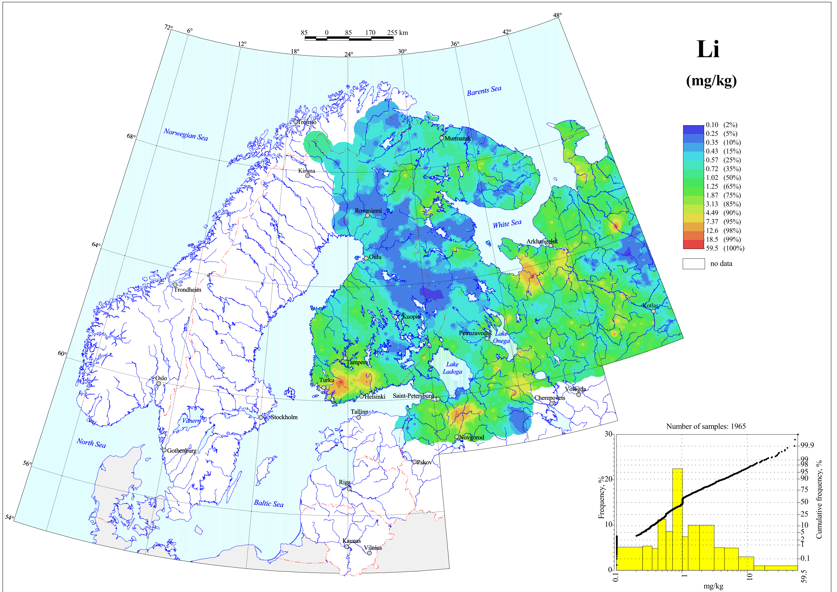
Lithium in Organic Soil Layer, Total Content
